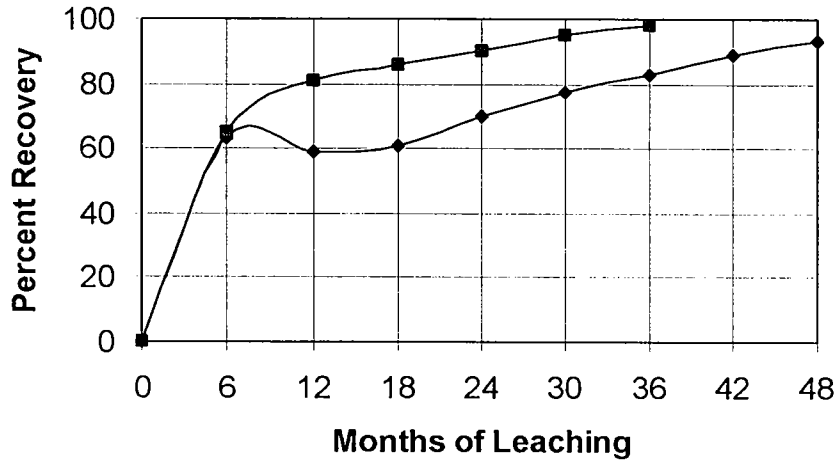
FIGURE 2. PERCENT RECOVERY OF TOTAL GOLD STACKED
