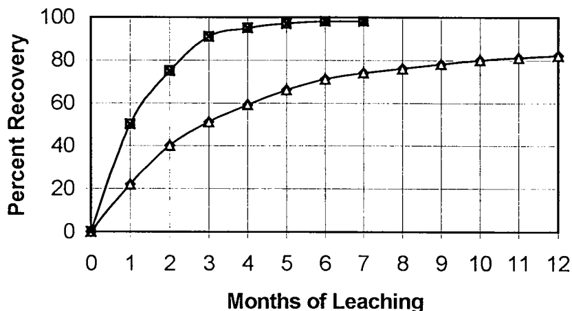
FIGURE 1. PERCENT RECOVERY OF TOTAL GOLD STACKED
