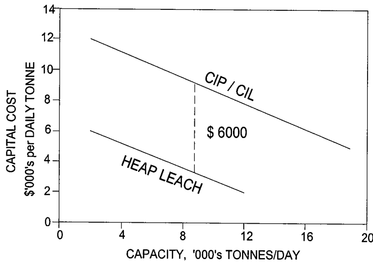
FIGURE 1. CAPACITY VERSUS CAPITAL COST
